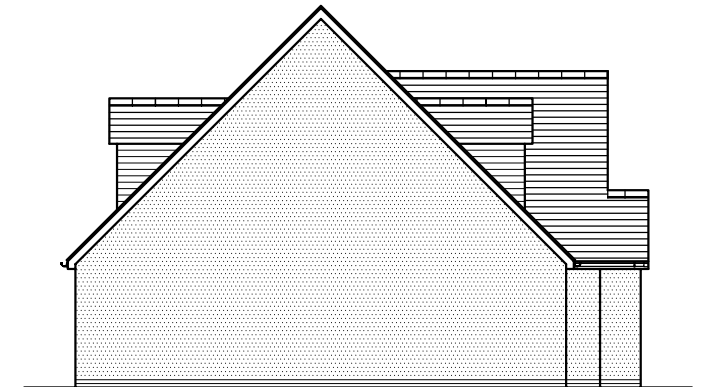
SIDE ELEVATION
