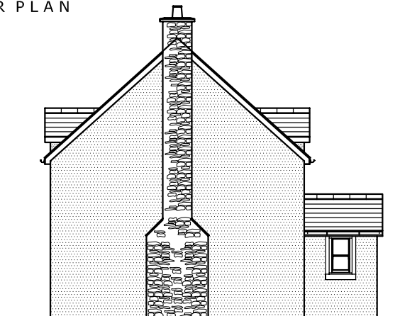
SIDE ELEVATION
